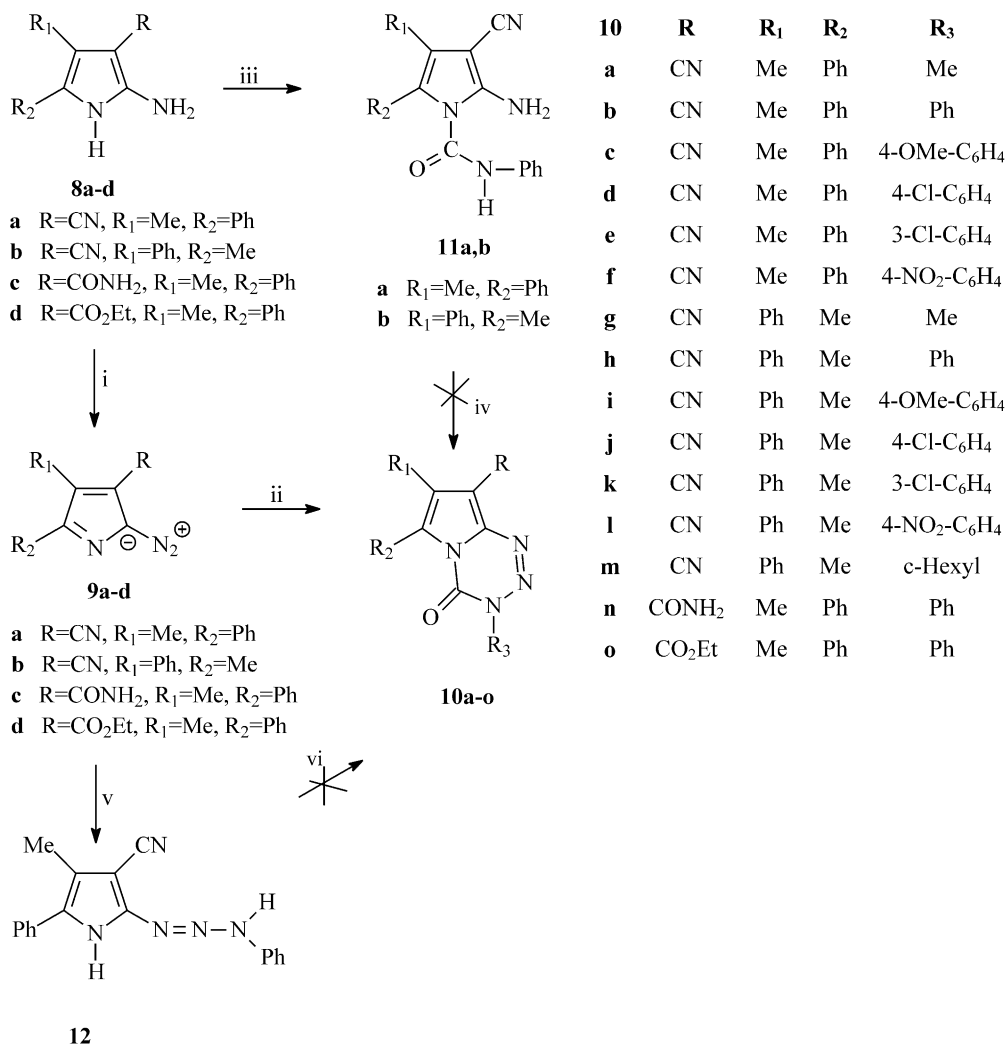
Scheme 2. Reagents: i NaNO 2 /CH 3 COOH, Na 2 CO 3 ; ii R 3 NCO/DMF; iii NaH/THF, PhNCO; iv NaNO 2 /H + ; v aniline/DCM; vi triphosgene or CDI/THF.
