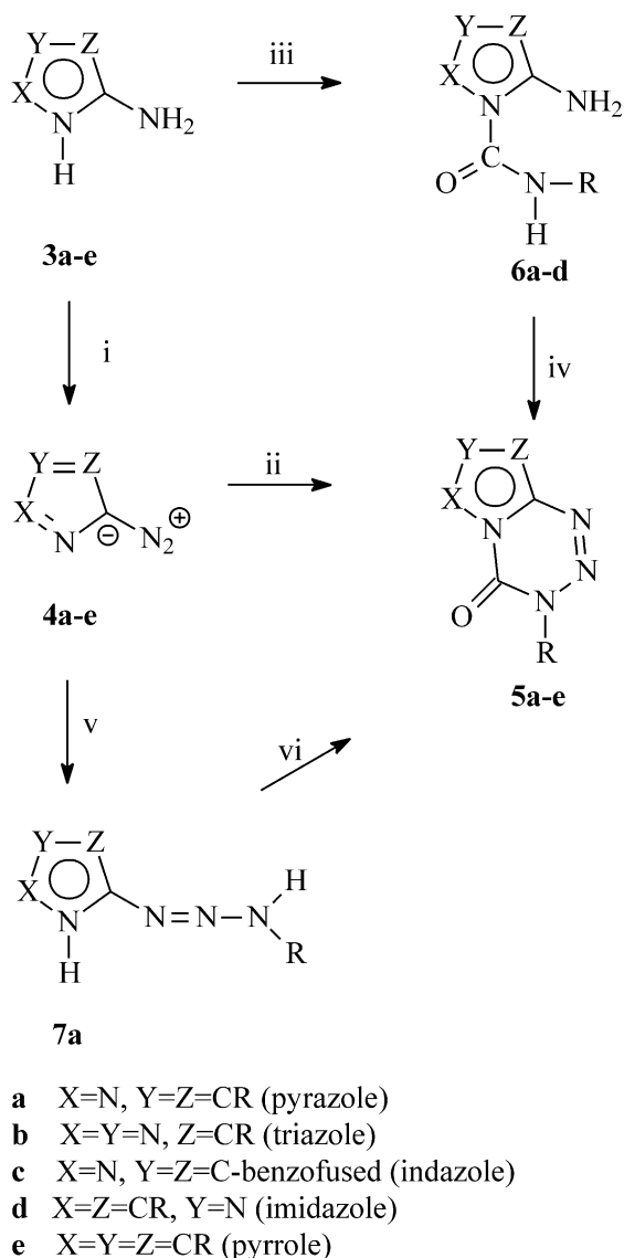
Scheme 1. Reagents: i \text{NaNO}_2/\text{H}^+ , \text{OH}^- ; ii \text{RNCO} ; iii \text{RNCO} or \text{ClCO}_2\text{Et}/\text{RNH}_2 or \text{RNHCOCl} ; iv \text{NaNO}_2/\text{H}^+ ; v \text{RNH}_2 ; vi \text{COCl}_2 or CDI.
